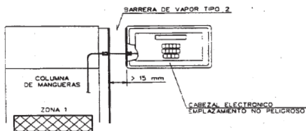
DETALLE "E"
