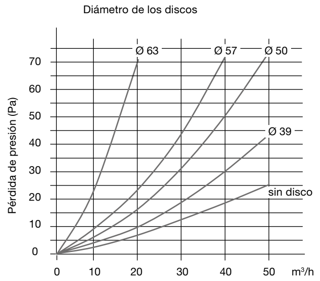
Zehnder ComfoTube 90
