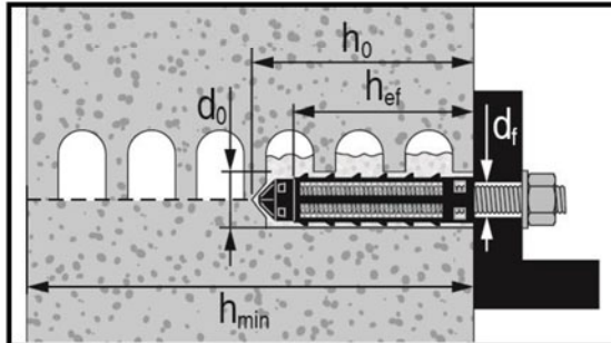
Figure A1: Hollow and solid brick with threaded rod, HIT-V... and one sieve sleeve HIT-SC (see Table B5), or with internally threaded sleeve HIT-IC and single sieve sleeve HIT-SC (see Table B7)
