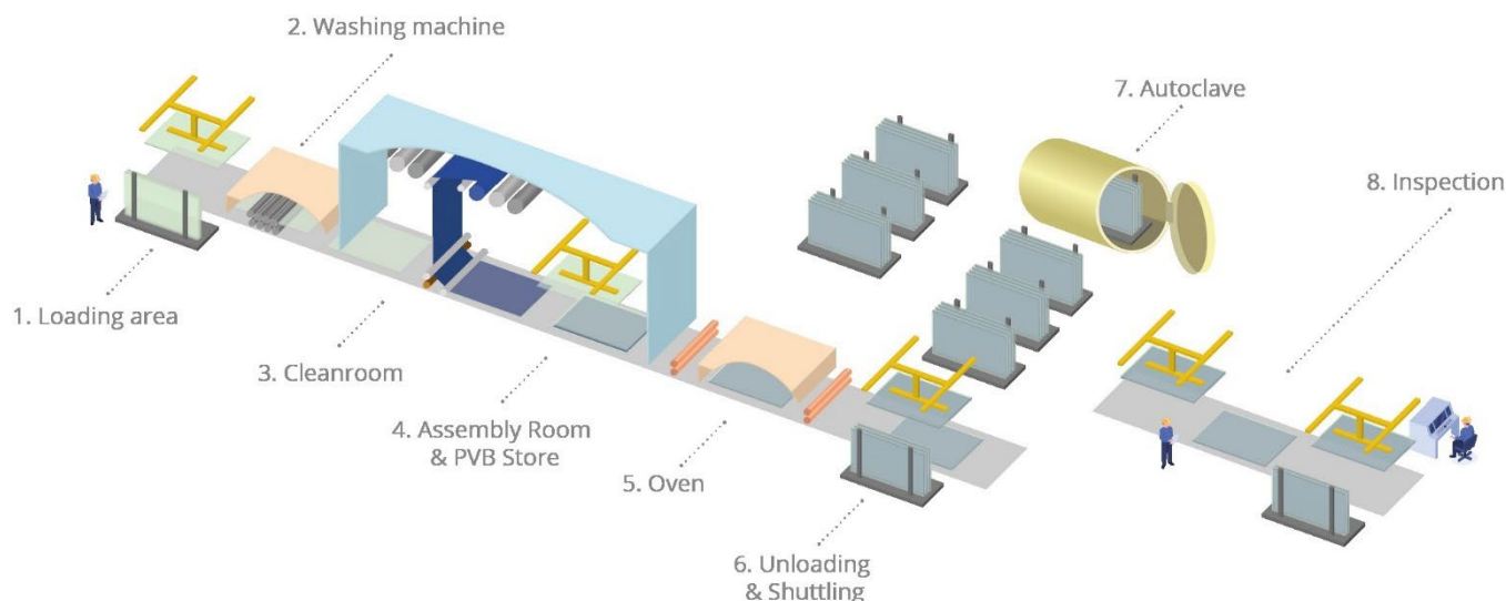
Figure 5 - Lamination Process
