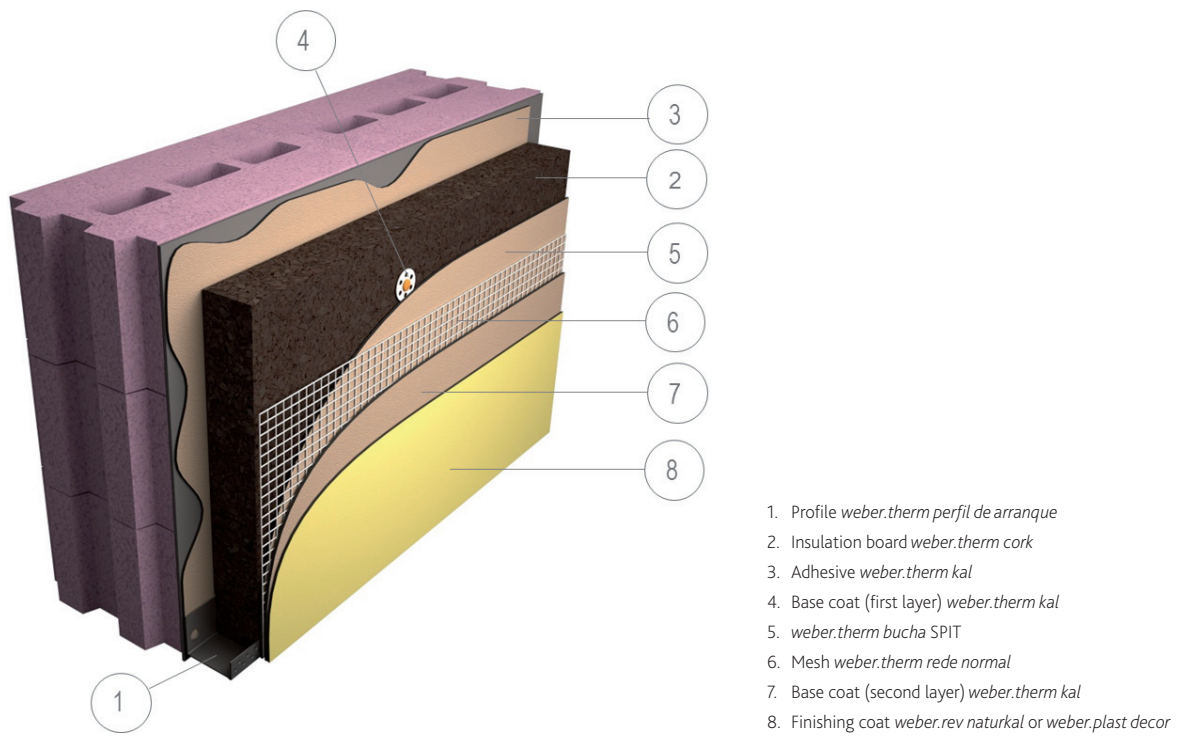
ETICS components
