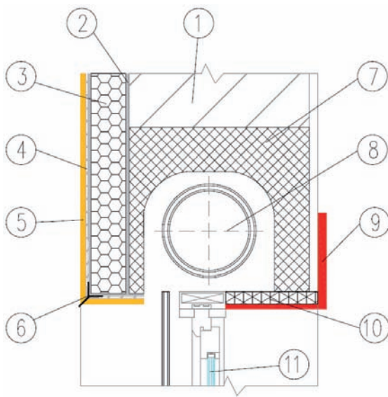
Vertical section of a window opening – Lintel with blind box
