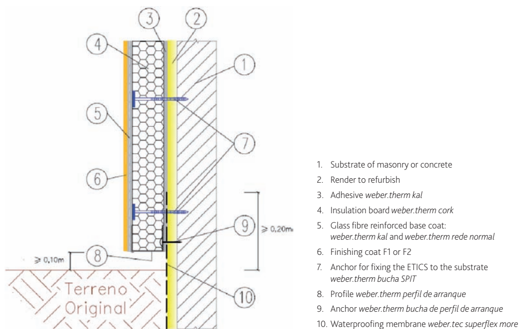
Vertical section of ETICS start
